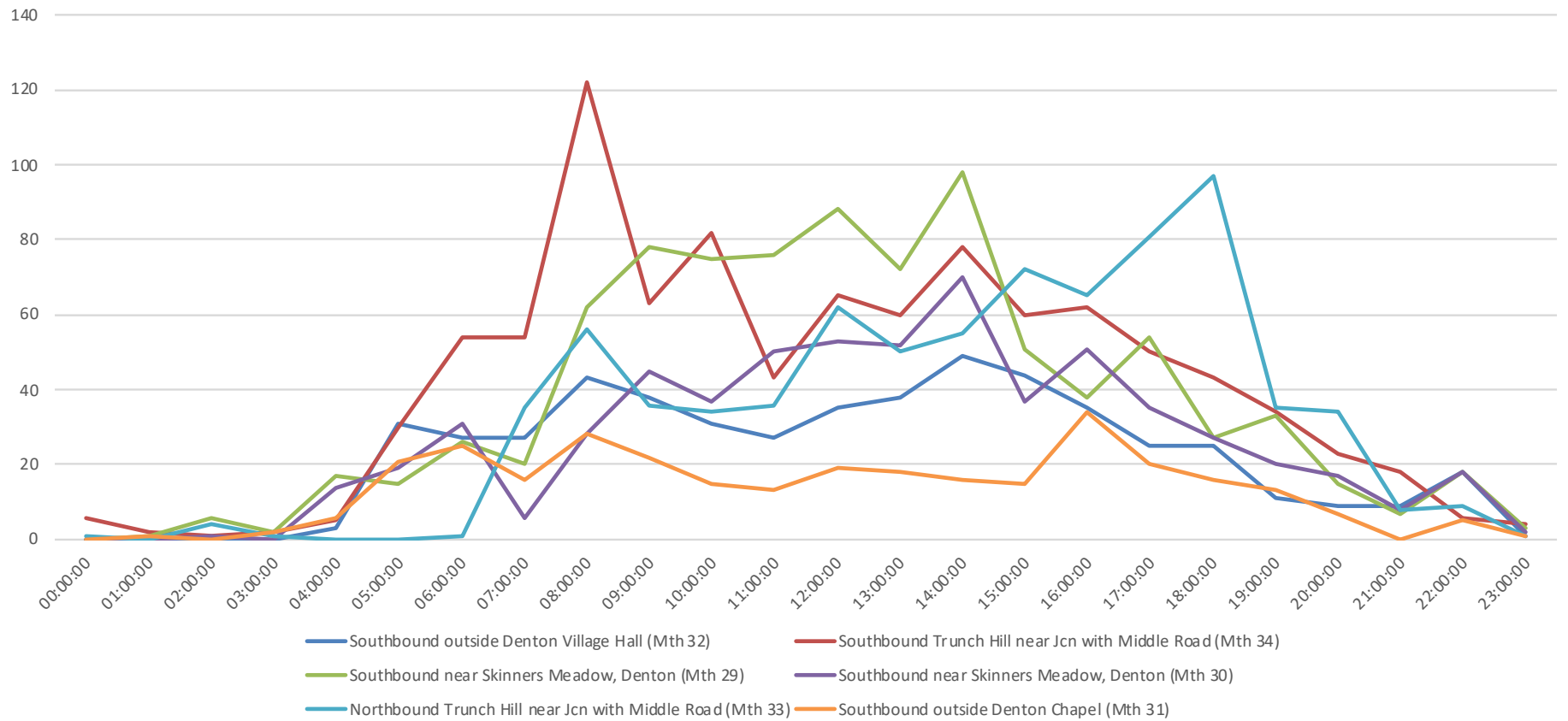
Number of Speeding Vehicles each hour over the month Dec 20 - May 21
