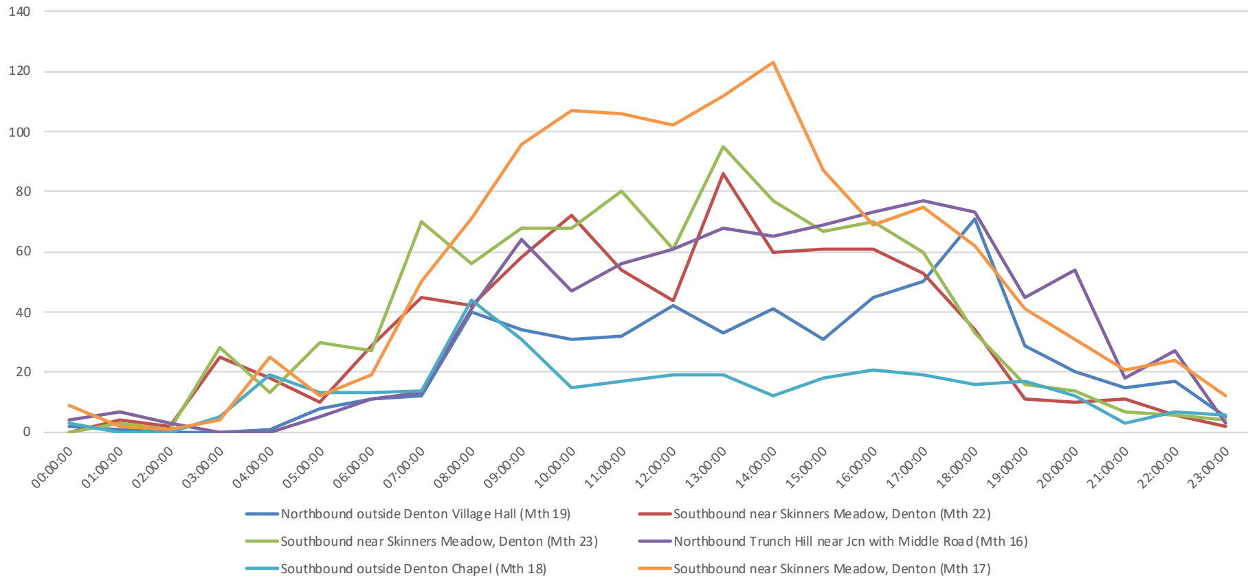
Number of Speeding Vehicles each hour over the month, in the last 8 months Nov 19-Jun 20
