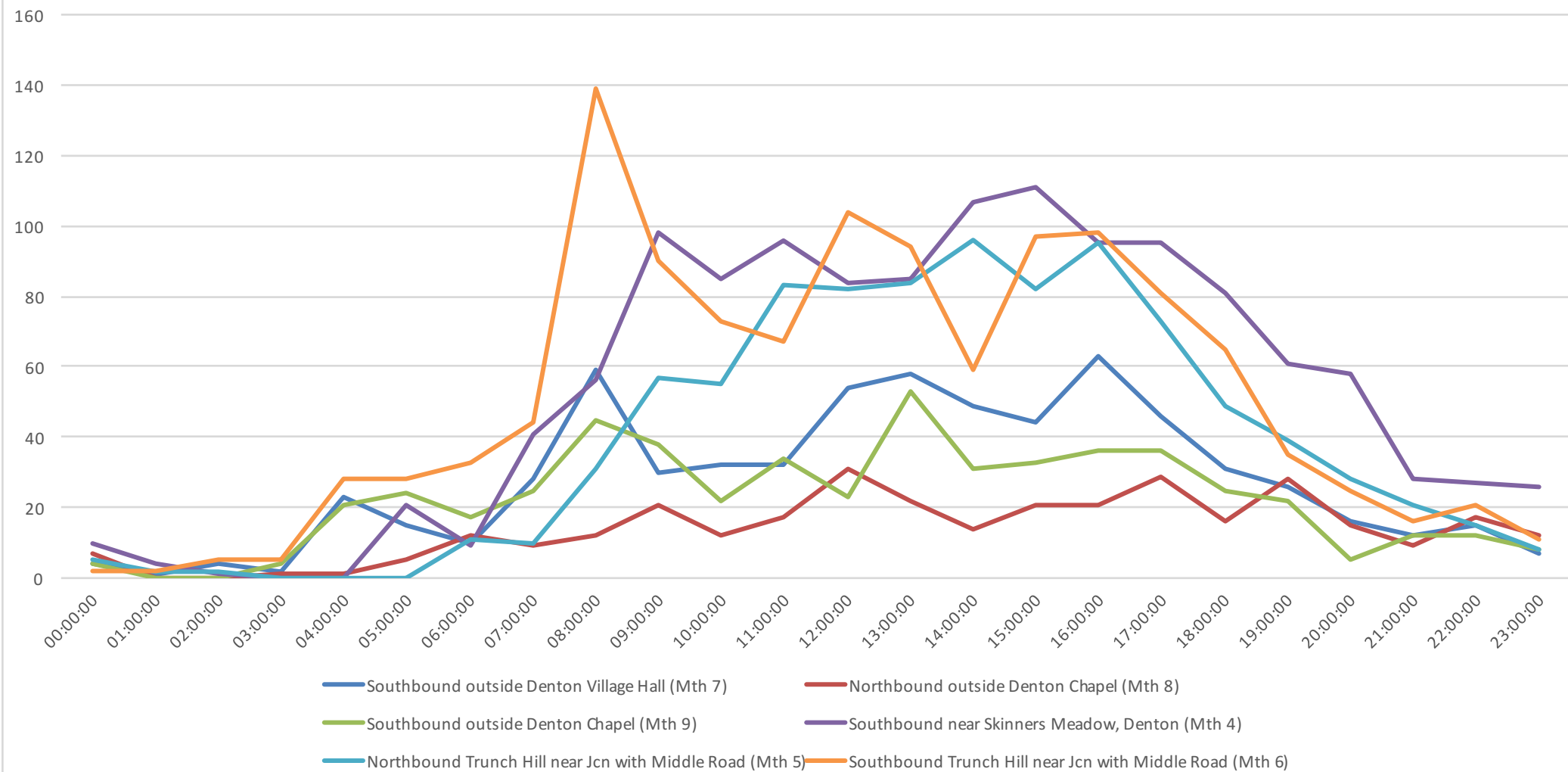
Number of Speeding Vehicles each hour over the month, in the last 6 months Nov18-Apr19
